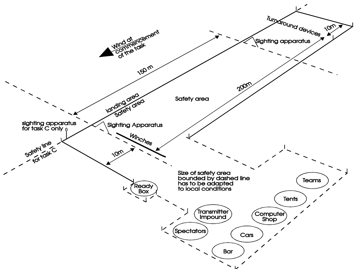
F3B FLYING FIELD LAYOUT
